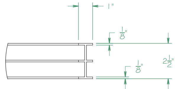
CROSS SECTION OF 1400 CHANNEL
