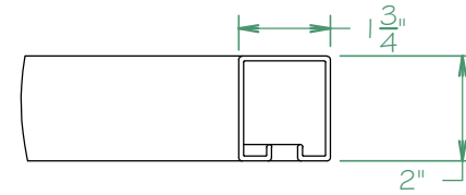
CROSS SECTION OF 1700 CHANNEL
